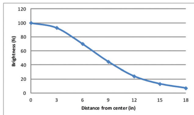
Photometrics: Light source placed 12.75" away from work surface
